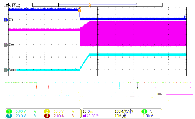
Figure 34. Shutdown remove
